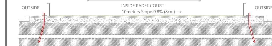
Cross section DETAIL A-A
